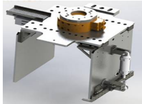
Customize Gripper
