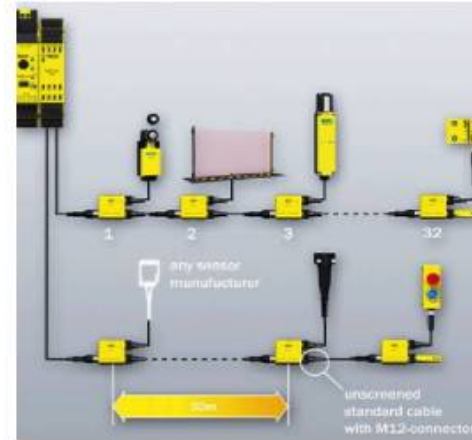
Safety Loop/Link
